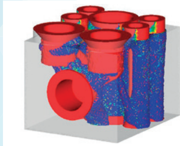
Fig. 1 Topology optimization result (element density color contour plot)
