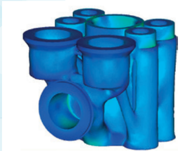
Fig. 3 Analysis of smoothed optimization design
