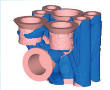
Fig. 2 Interpretation and remesh of topology optimization result
